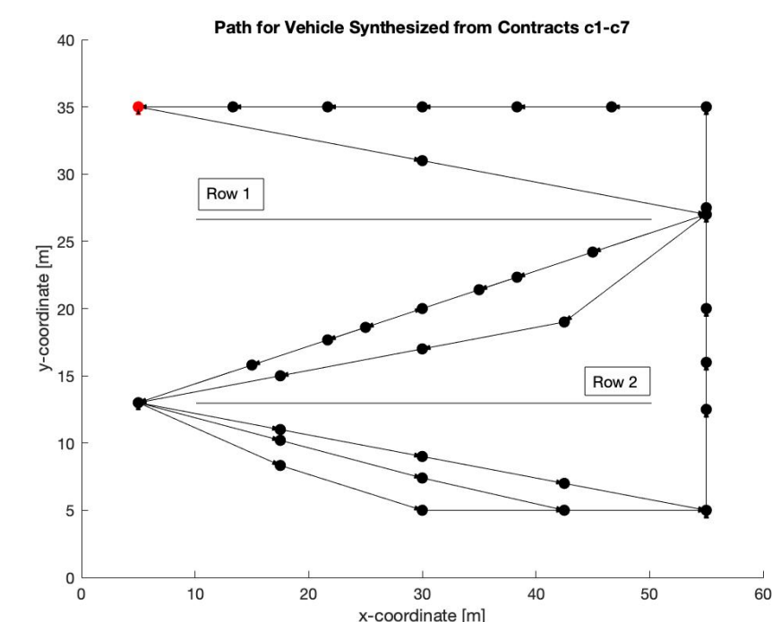
Figure 5: Autonomous Vehicle Control from Contracts
