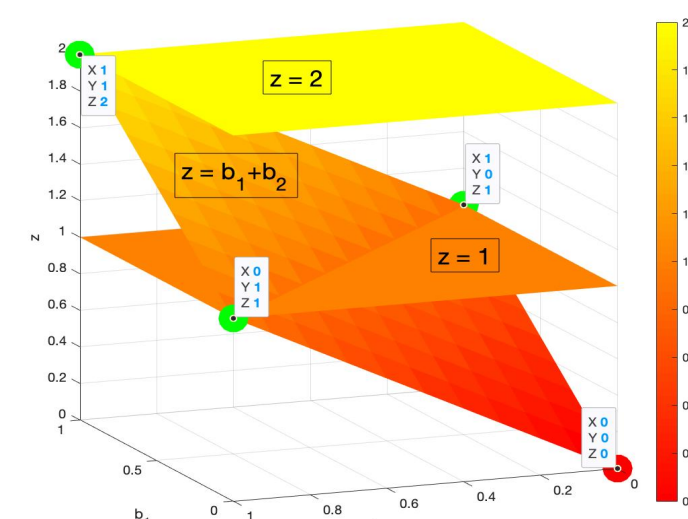
Figure 3: "OR" Constraints
