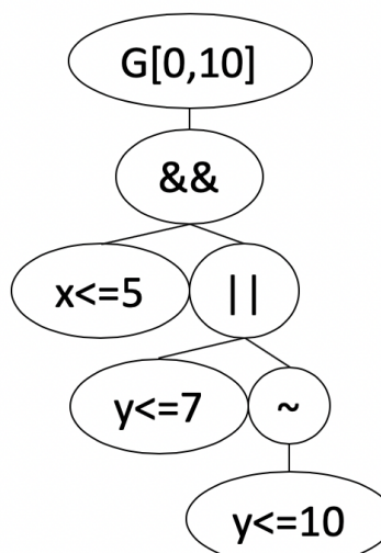
Figure 2: STL Tree
